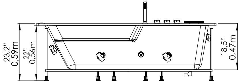
VISTA LATERAL / LATERAL VIEW
