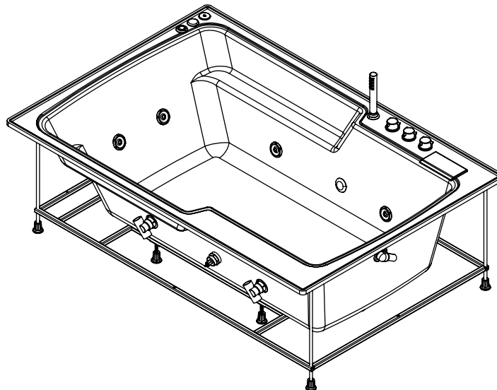
VISTA ISOMÉTRICA / ISOMETRIC VIEW
