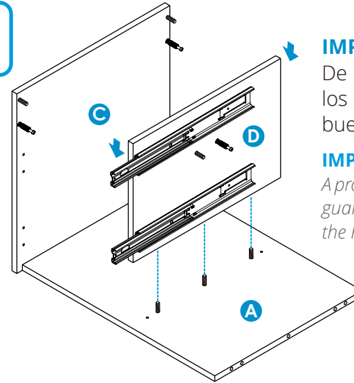
Riel full extensión liviano Lightweight full extension rail
