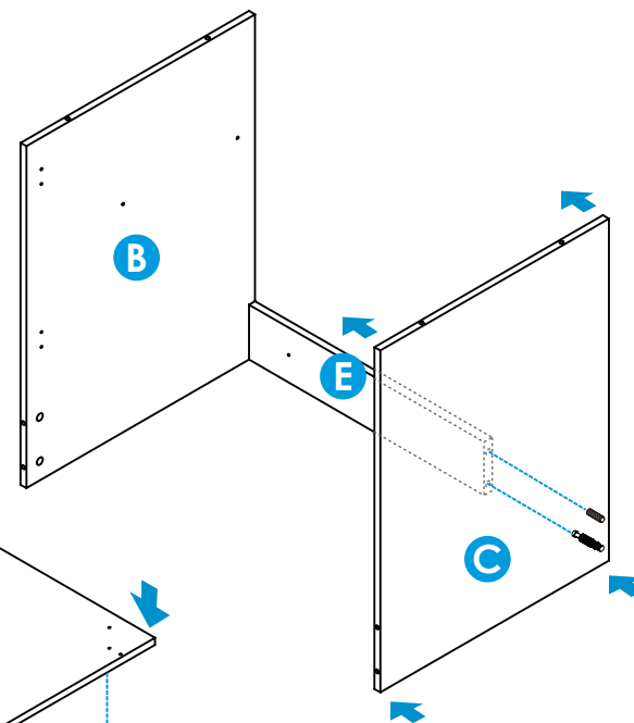
Tornillos ensamble 2" Assembly screws 2"
